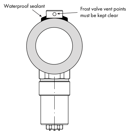
Figure 3-21: Insulated Frost Valve end view
