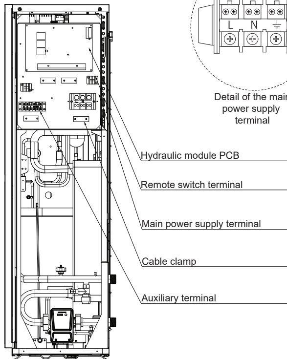
Figure 6-2: Side view for Mains and Hydraulic PCB connection
