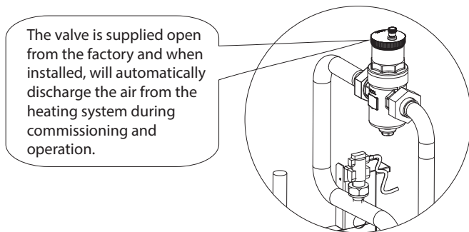
Figure 4-1: Automatic Air Vent
