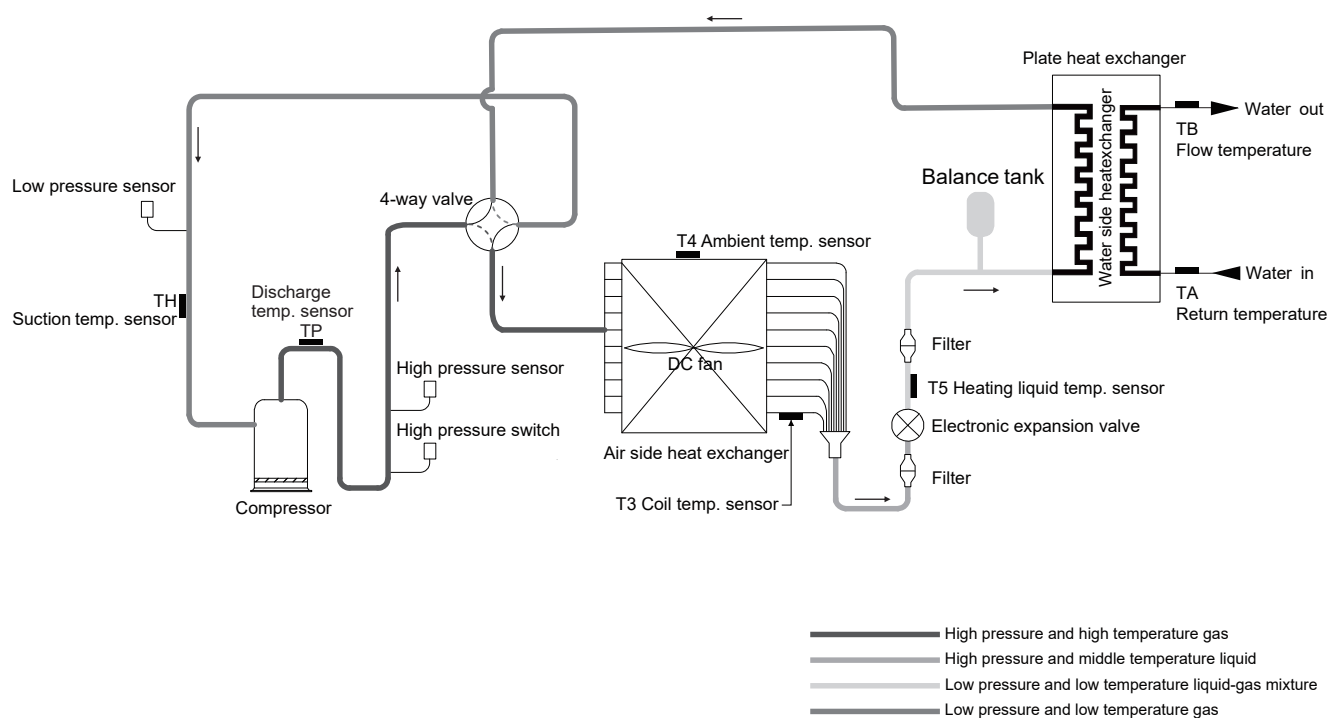
Figure 8-2: Refrigerant flow - Defrost
