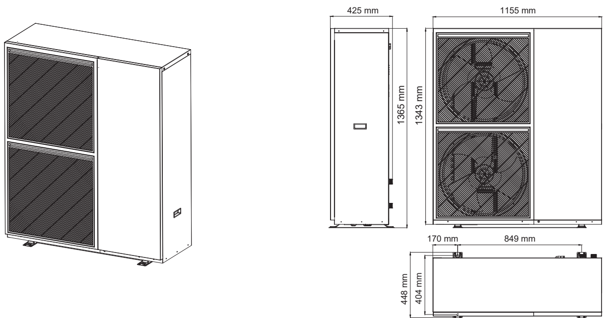
Figure 2-3: HPR290i120 & HPR290i160 heat pump dimensions
