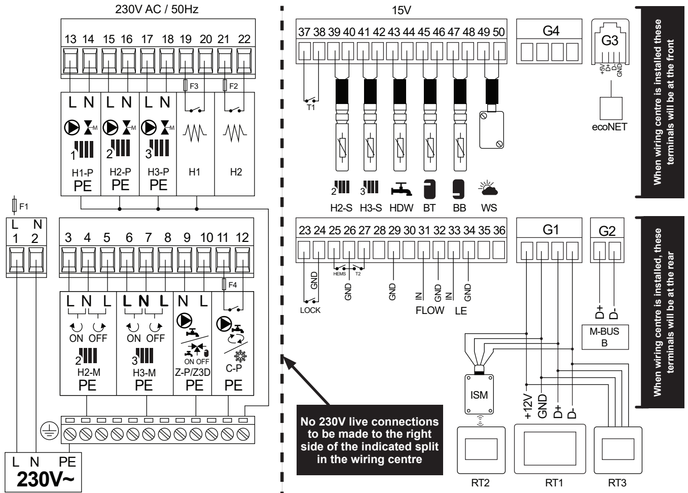
Figure 6-7: Wiring centre - Terminals
