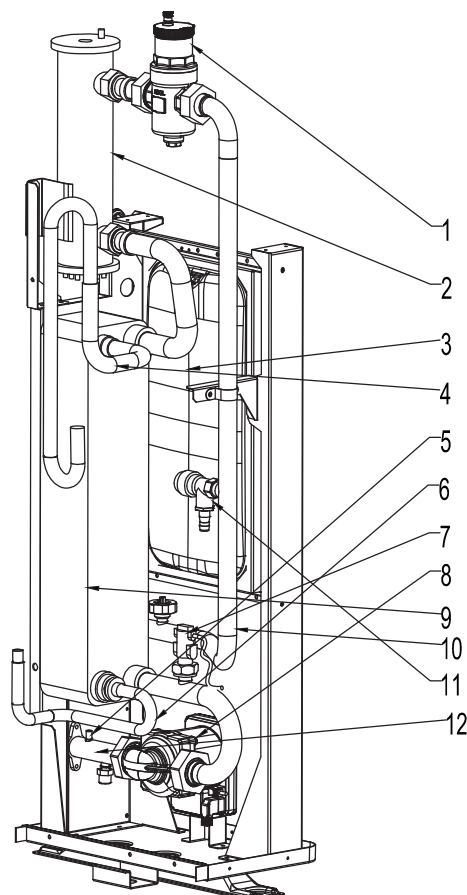
Figure 1-8: Hydraulic module - 12kW & 16kW
