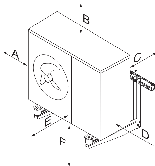
Figure 3-15: Wall mounted installation clearances
