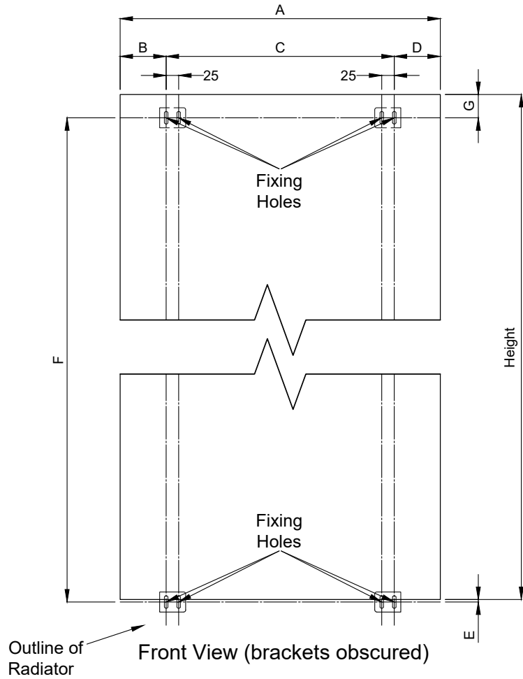
Figure 3-6: Fixing hole positions for Vertical radiators
