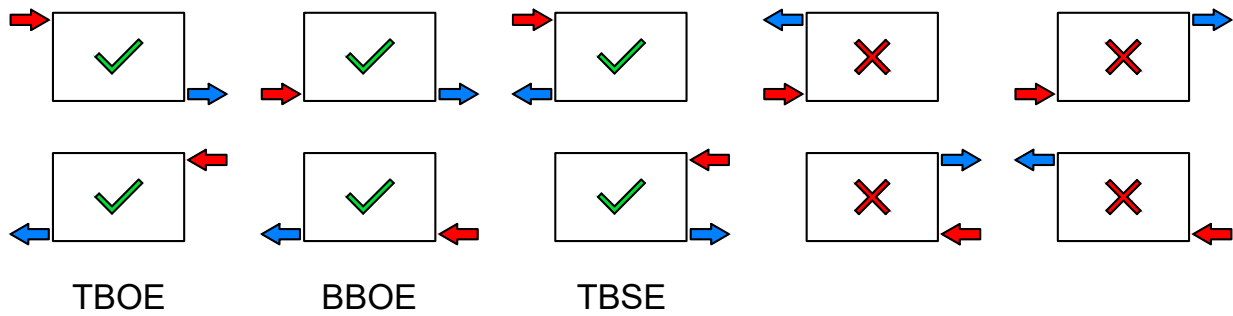
Figure 3-2: Pipe Connection Options
