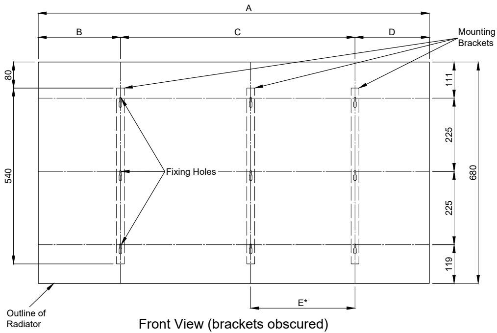
Figure 3-5: Fixing hole positions for Horizontal 680mm high radiators
