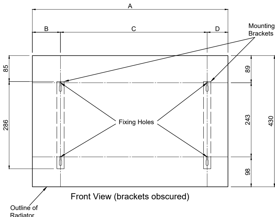
Figure 3-3: Fixing hole positions for Horizontal 430mm high radiators
