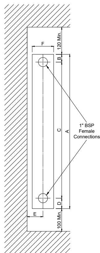
Figure 3-1: Radiator Clearances and Dimensions
