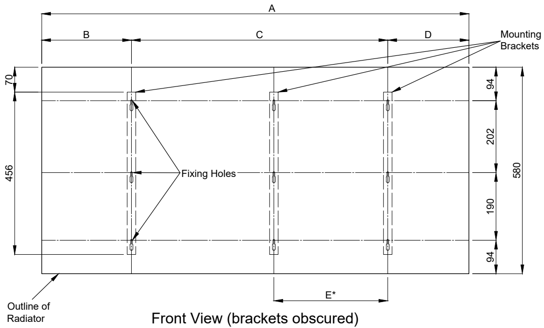
Figure 3-4: Fixing hole positions for Horizontal 580mm high radiators
