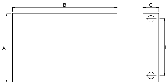
Figure 2-1: Radiator Dimensions
